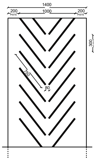
NT L 1400 MM
